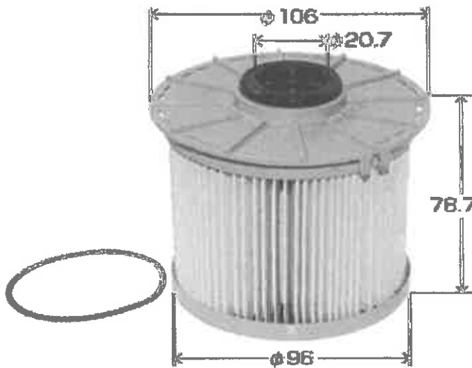
略図 Brief Drawing
