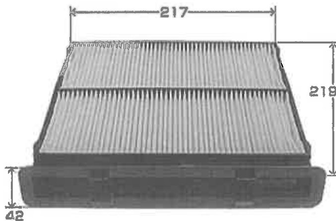
略図 Brief Drawing
