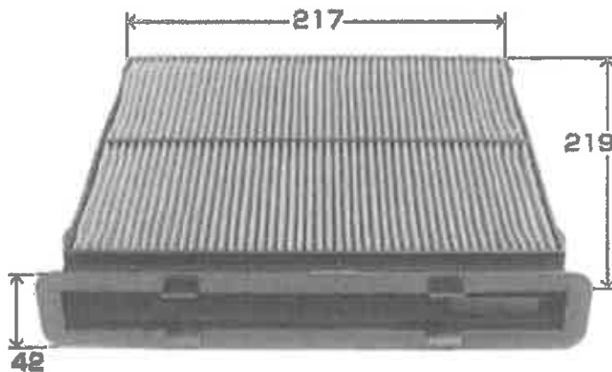
略図 Brief Drawing
