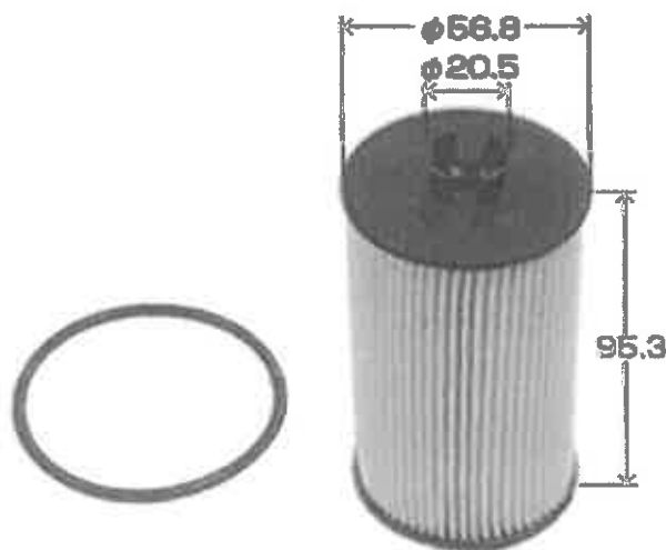
略図 Brief Drawing
